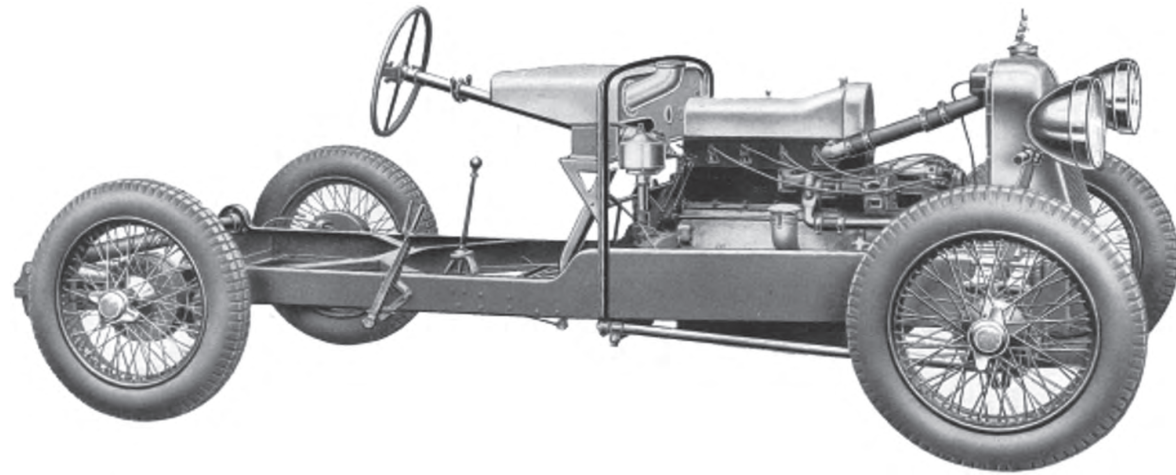
FRONT-WHEEL DRIVE CHASSIS
