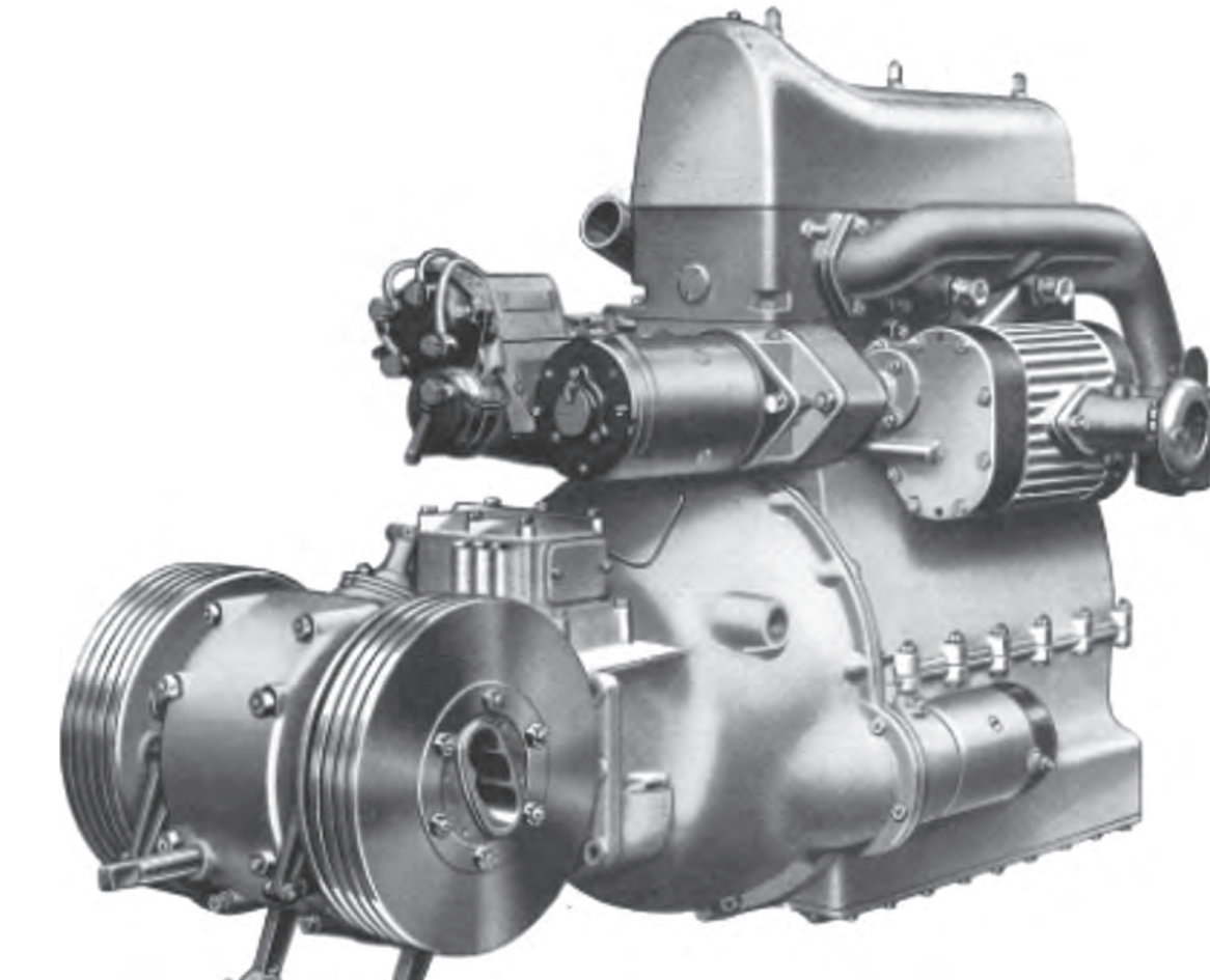
THE ALVIS FRONT WHEEL DRIVE UNIT
